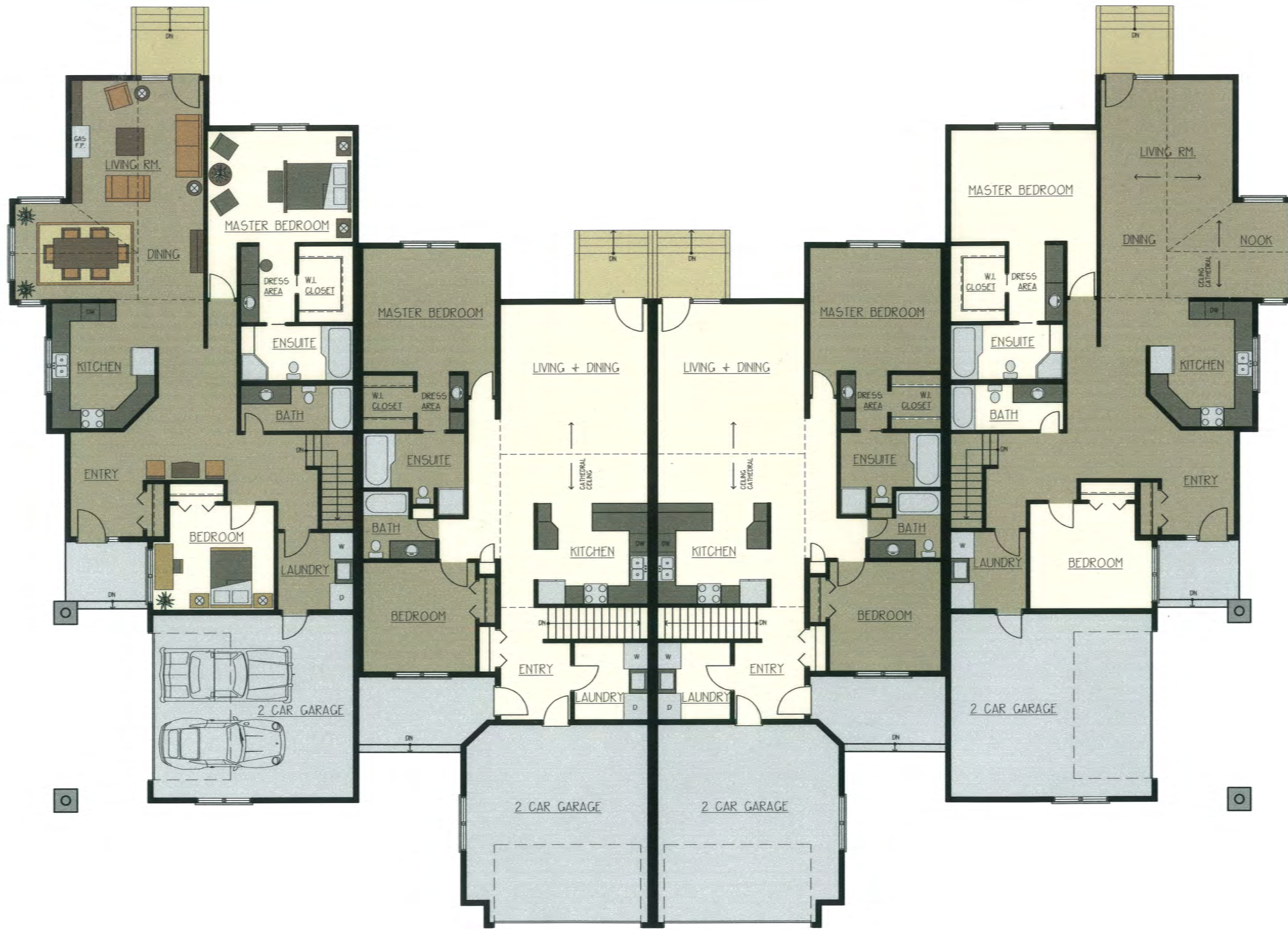
KING GEORGE'S PARK Luxury Townhomes Main Floor Plan
